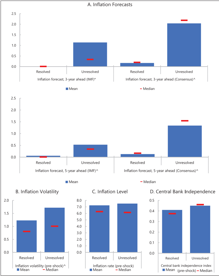
Figure 11. Inflation Anchoring
