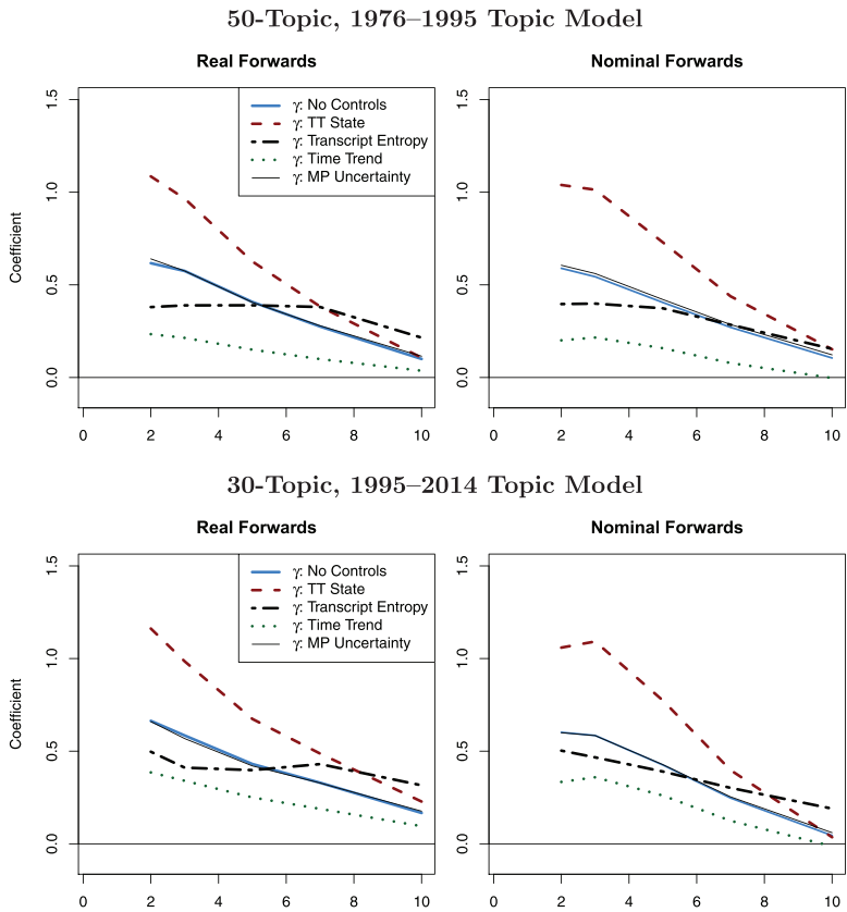
Figure F.2. Robustness of Regression Results to K and Sample Period
