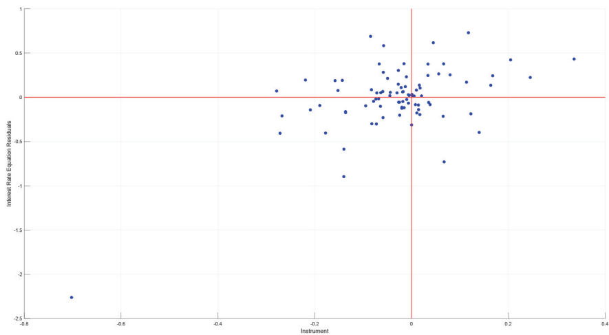
Figure C.2. Baseline Model Interest Rate Equation Residuals and Instrumental Surprises
