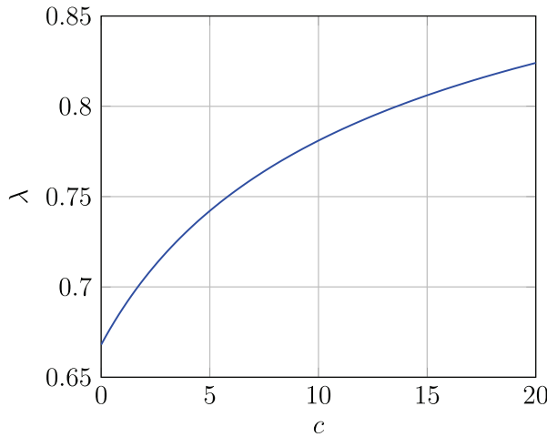
Figure A.1. \lambda as a Function of c , when \mathbb{I}_{t+2}^i = 1
