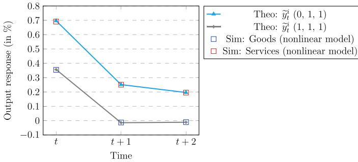
Figure A.3. Comparing Theoretical vs. Simulated Output Responses to a 1 Percent One-Time Expansionary Monetary Policy Shock at t = 1 ( c = 10 , AR1 reallocation shock \rho = 0.9 )
