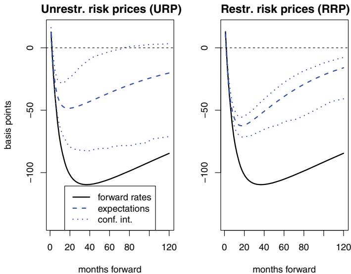
Figure 3. Shift of Forward Curve and Policy Path: URP vs. RRP
