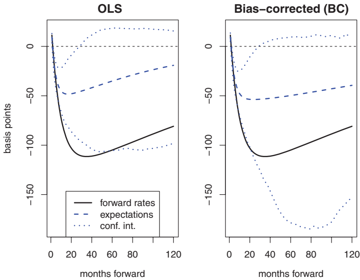
Figure 2. Shift of Forward Curve and Policy Path: OLS vs. BC
