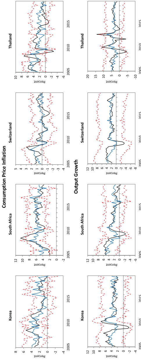
Figure 5. Conditional Quantiles
